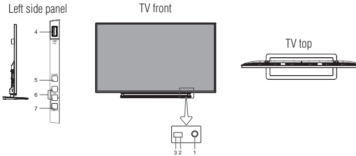
(Sample Illustration)58/65L5400U - Front and side panel controls and connection
